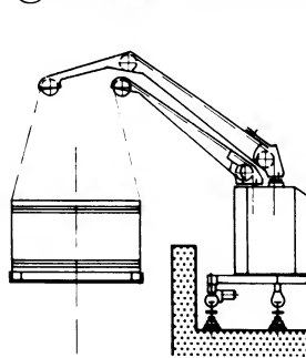
10 With two independently operated jibs
